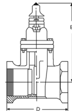
8057 Threaded Ends 2"-3"
